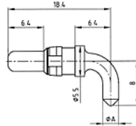
Plug premating
