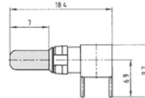
Plug premating
