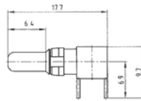
Plug premating
