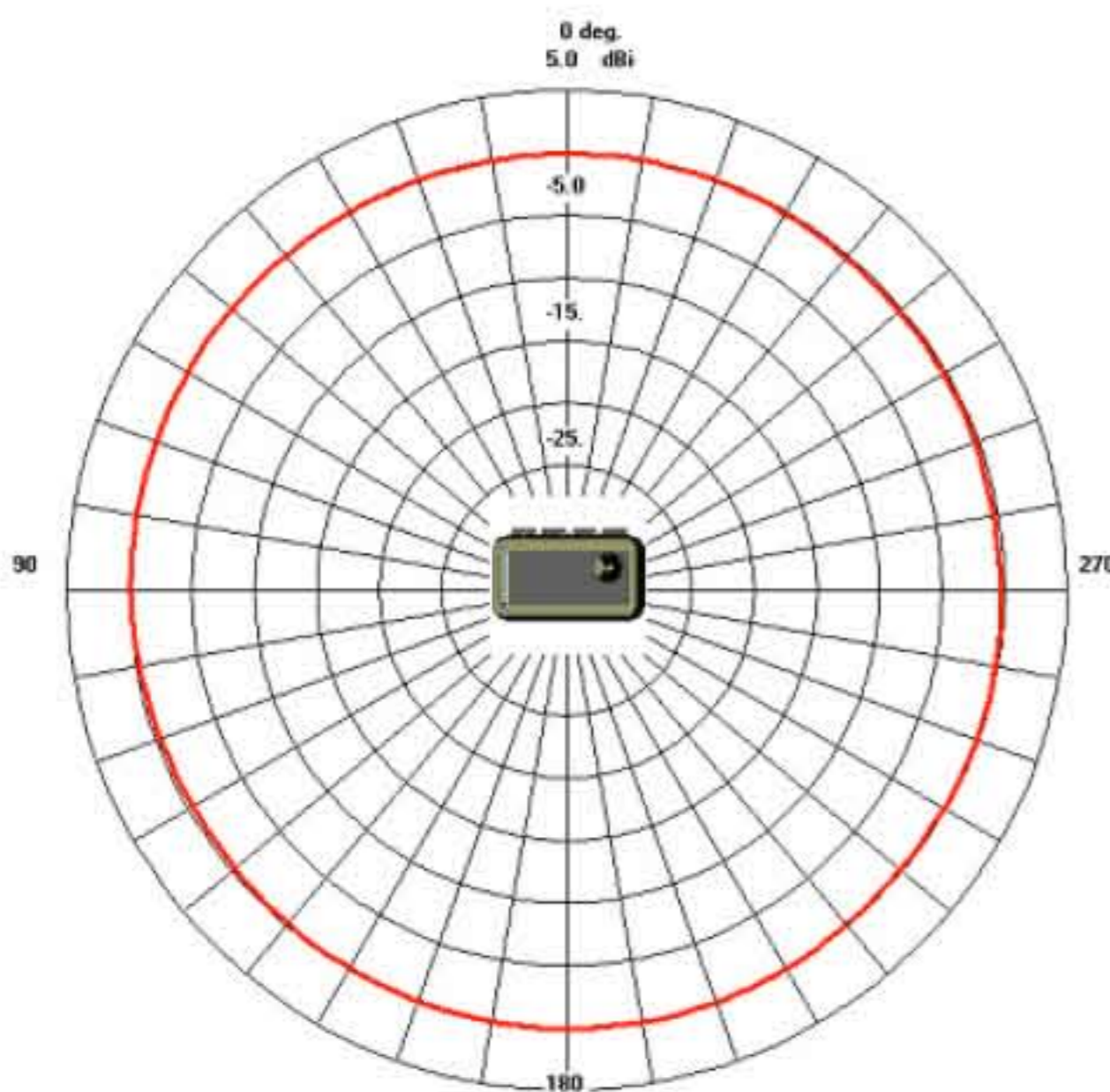
Azimuth EXR2400-TNSP
